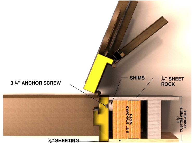
STANDARD DOOR INSTALLATION (TOP VIEW)
