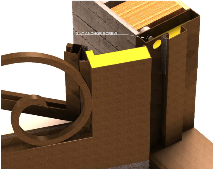
STANDARD DOOR INSTALLATION (SIDE VIEW)
