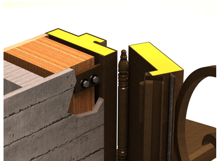
INTERIOR TAB MOUNT (SIDE VIEW)
